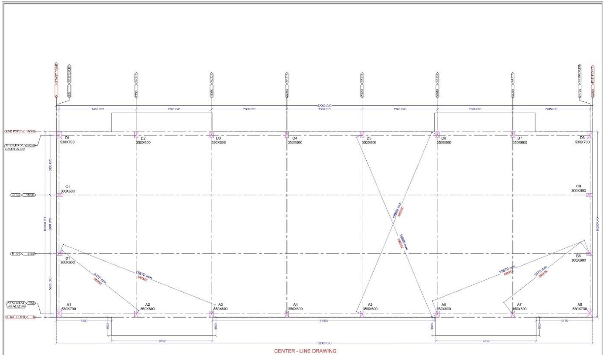
CENTER - LINE DRAWING
